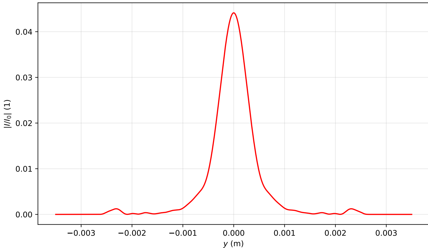
Intensity profile I(x = 0, y, z = 3.503)/I_0 , P_{in}=20.0P_{cr} , artificial time
