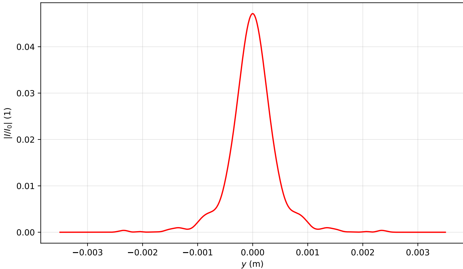
Intensity profile I(x = 0, y, z = 3.662)/I_0 , P_{in}=20.0\text{Pcr} , artificial time
