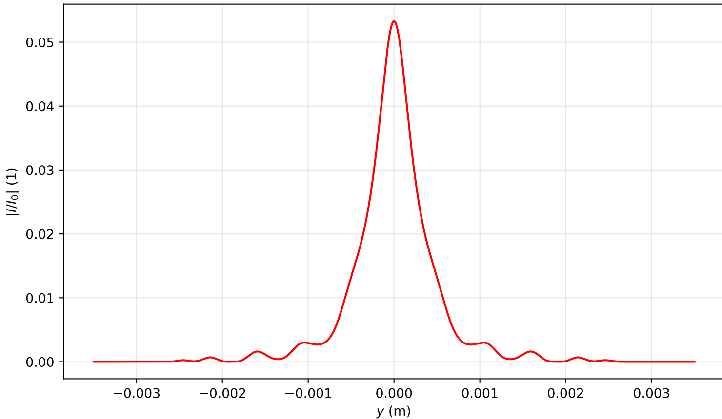
Intensity profile I(x=0, y, z=3.821)/I_0 , P_{in}=20.0P_{cr} , artificial time
