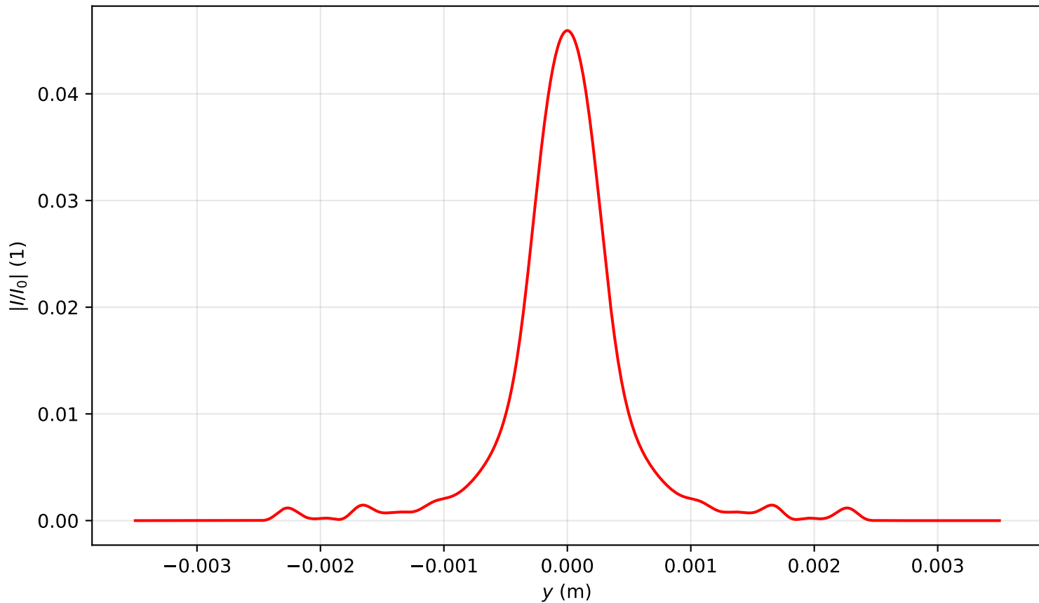
Intensity profile I(x=0, y, z=3.981)/I_0 , P_{in}=20.0\text{Pcr} , artificial time
