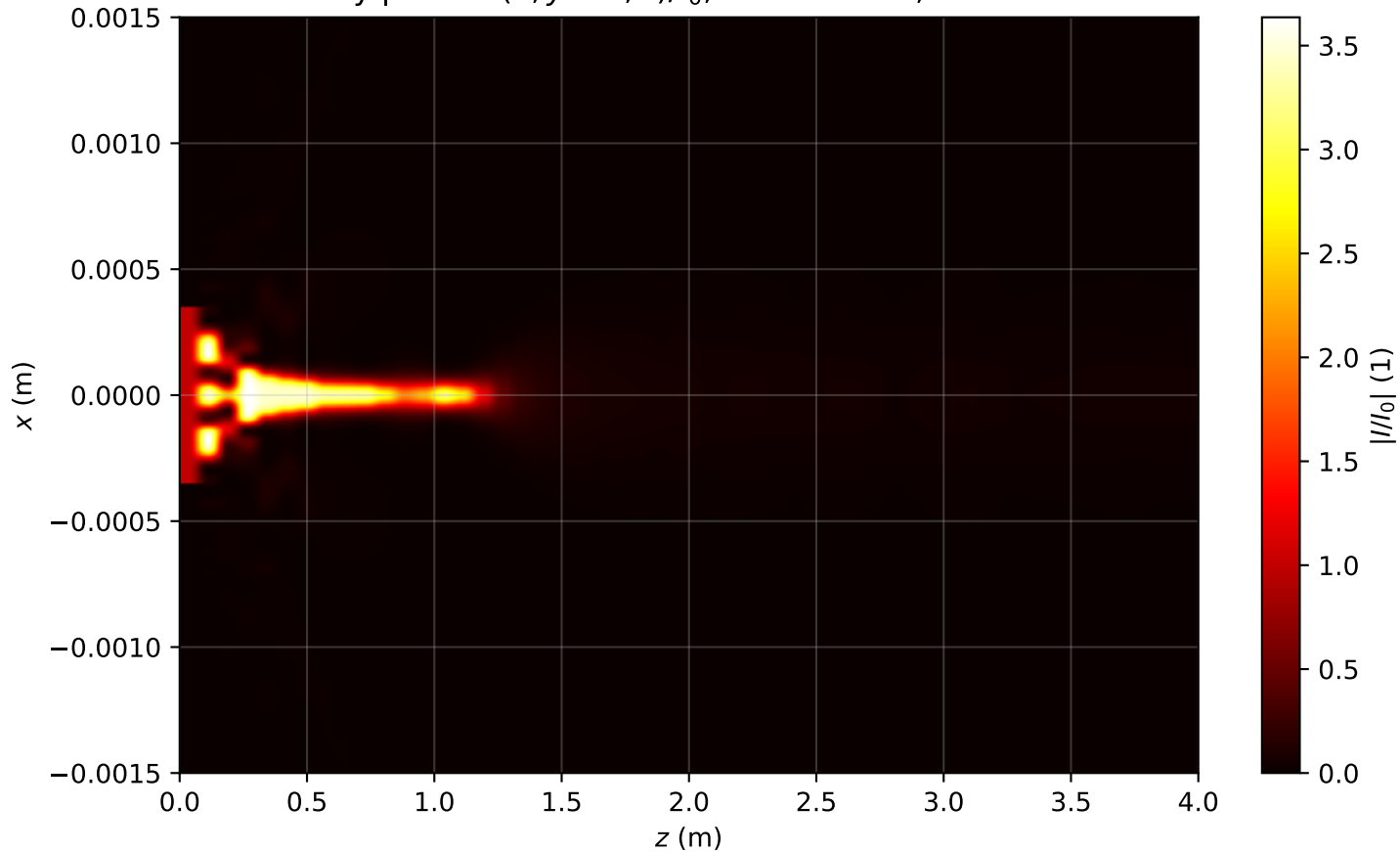
Intensity profile I(x, y = 0, z)/I_0 , P_{in}=20.0P_{cr} , artificial time
