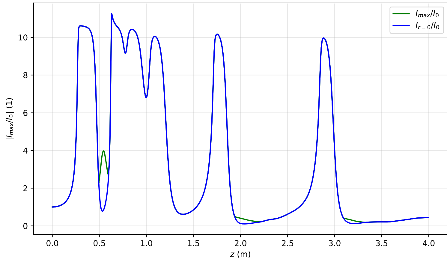
I_{\max}(x = 0, y = 0, z)/I_0 , Pin=10.5Pcr, artificial time
