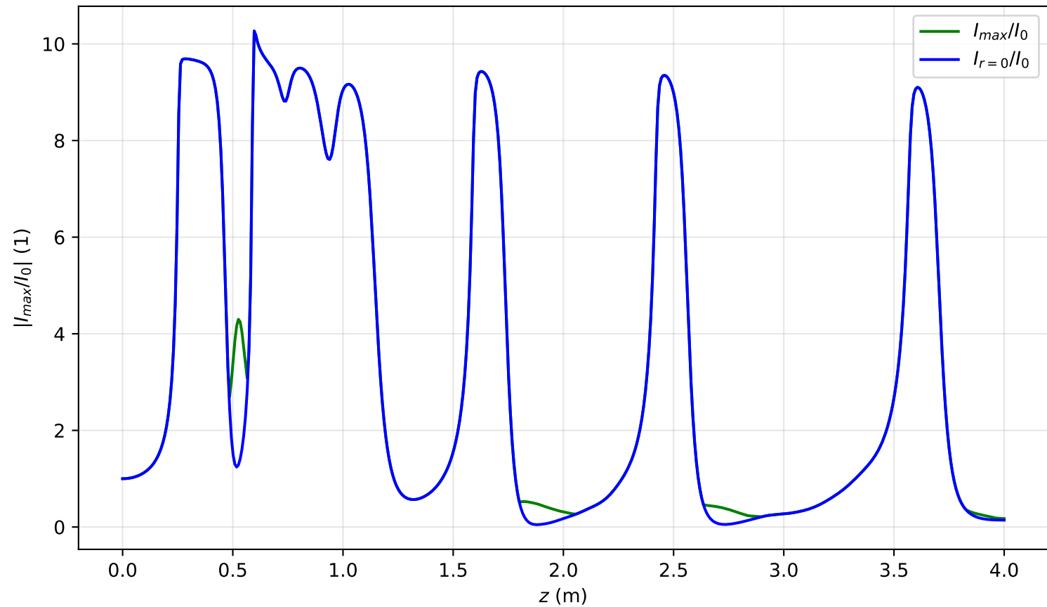
I_{\max}(x = 0, y = 0, z)/I_0 , Pin=11.5Pcr, artificial time
