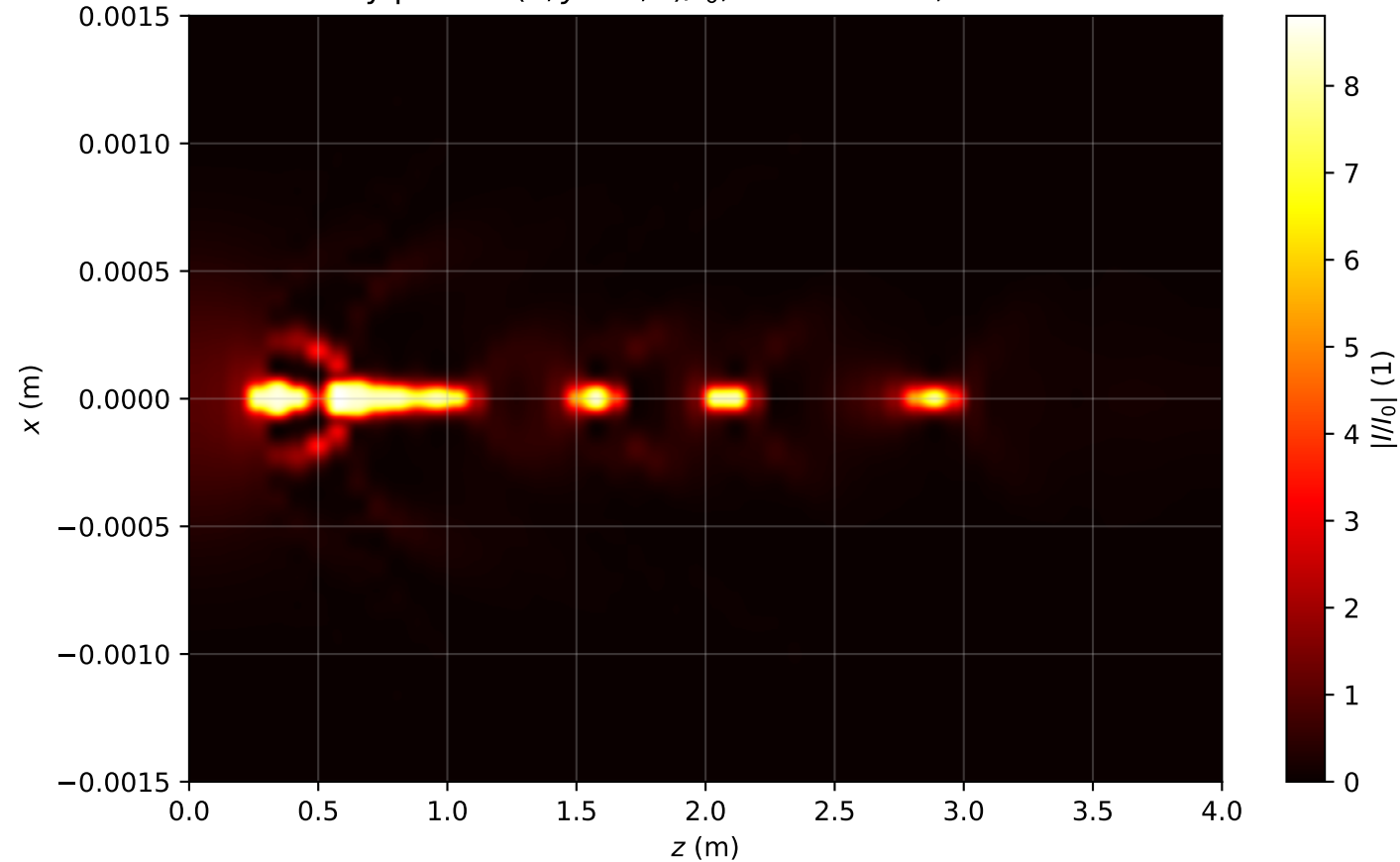
Intensity profile I(x, y = 0, z)/I_0 , P_{in}=13.0\text{Pcr} , artificial time
