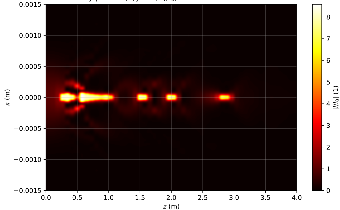
Intensity profile I(x, y = 0, z)/I_0 , P_{in}=13.5\text{Pcr} , artificial time
