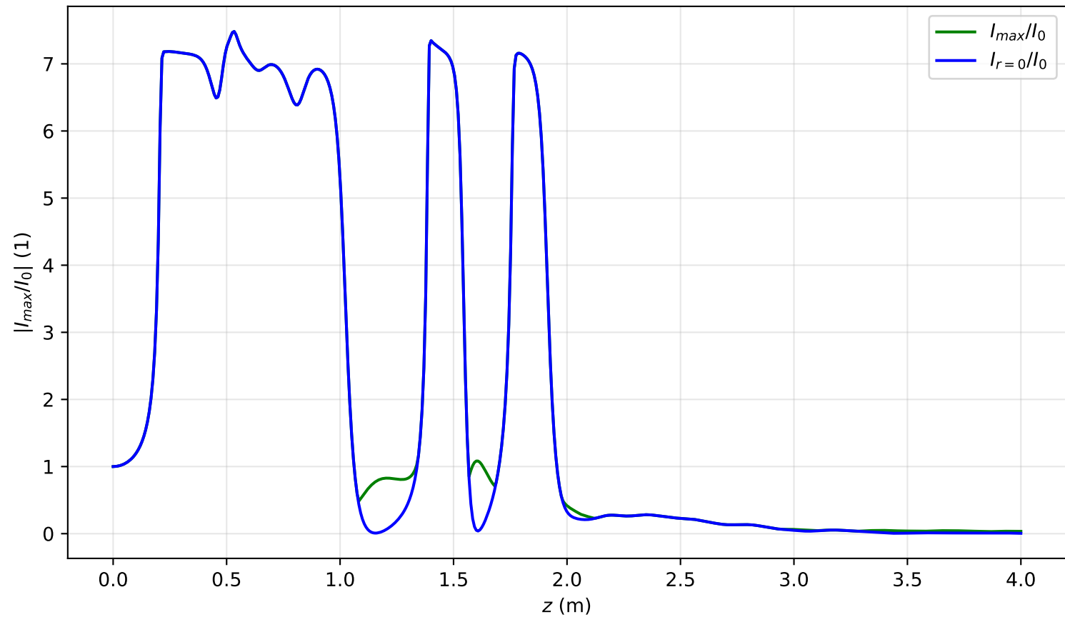
I_{max}(x = 0, y = 0, z)/I_0 , Pin=15.5Pcr, artificial time
