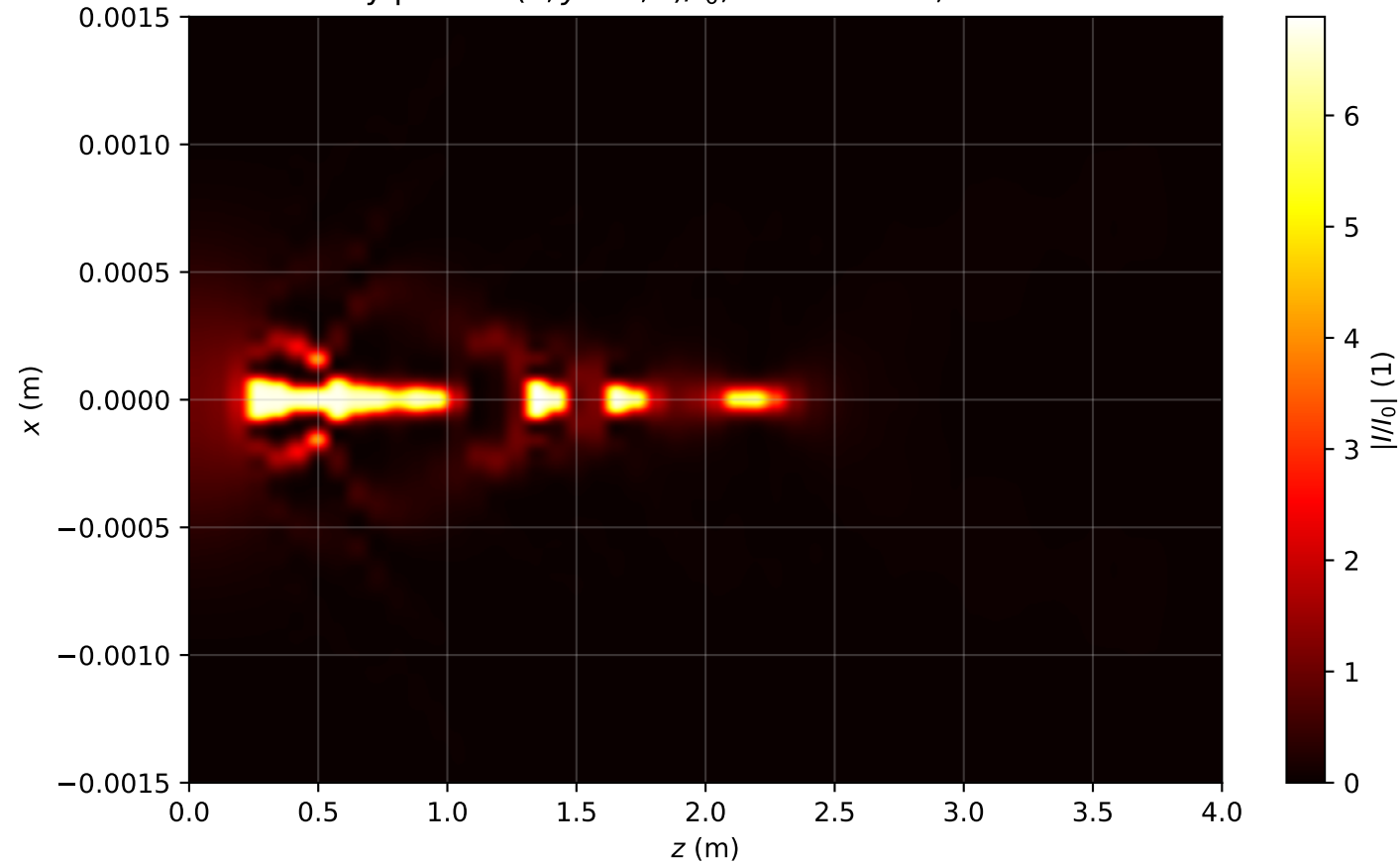
Intensity profile I(x, y = 0, z)/I_0 , P_{in}=16.5P_{cr} , artificial time
