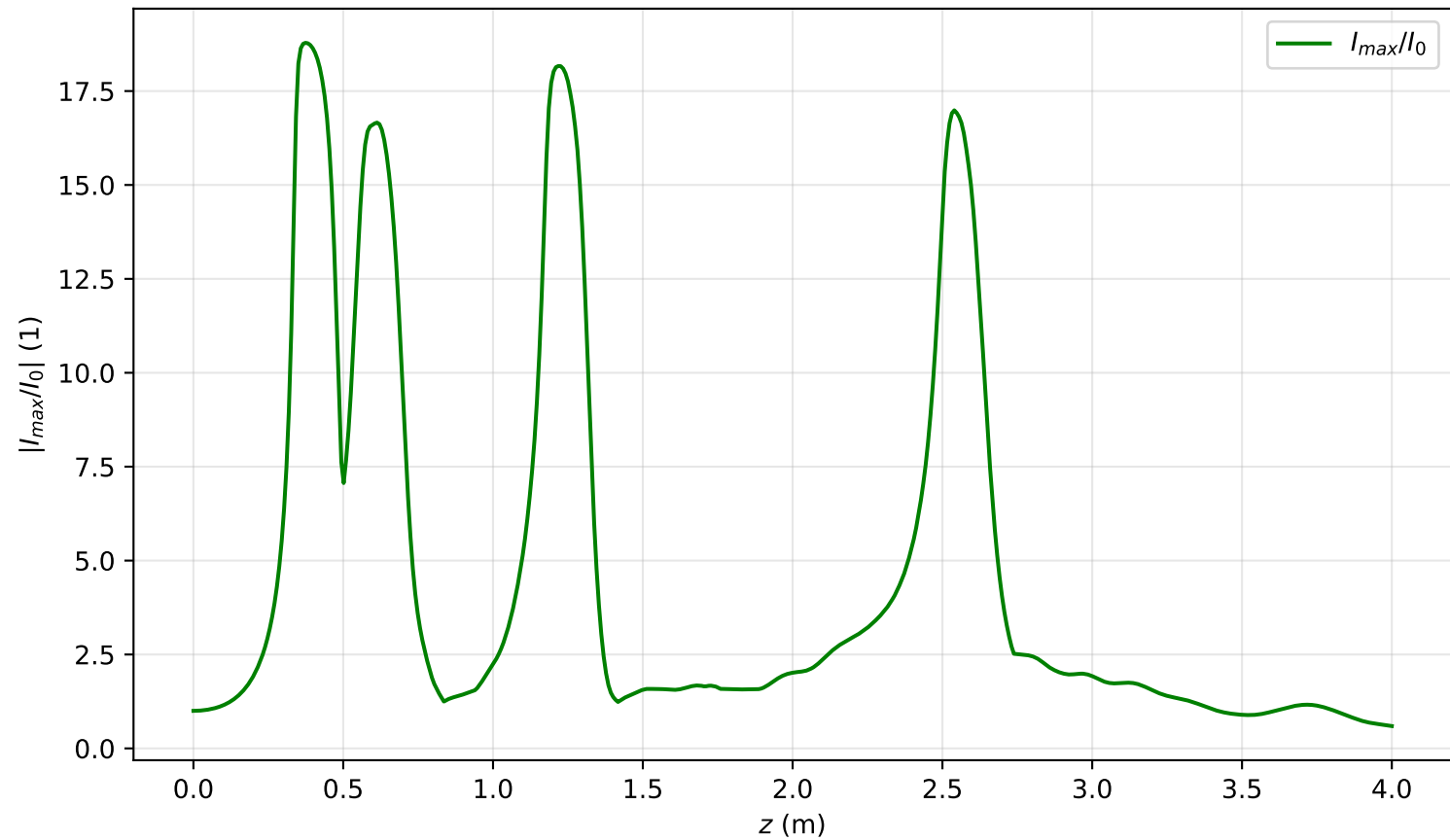
I_{\max}(x=0, y=0, z)/I_0 , Pin=12.0Pcr, artificial time
