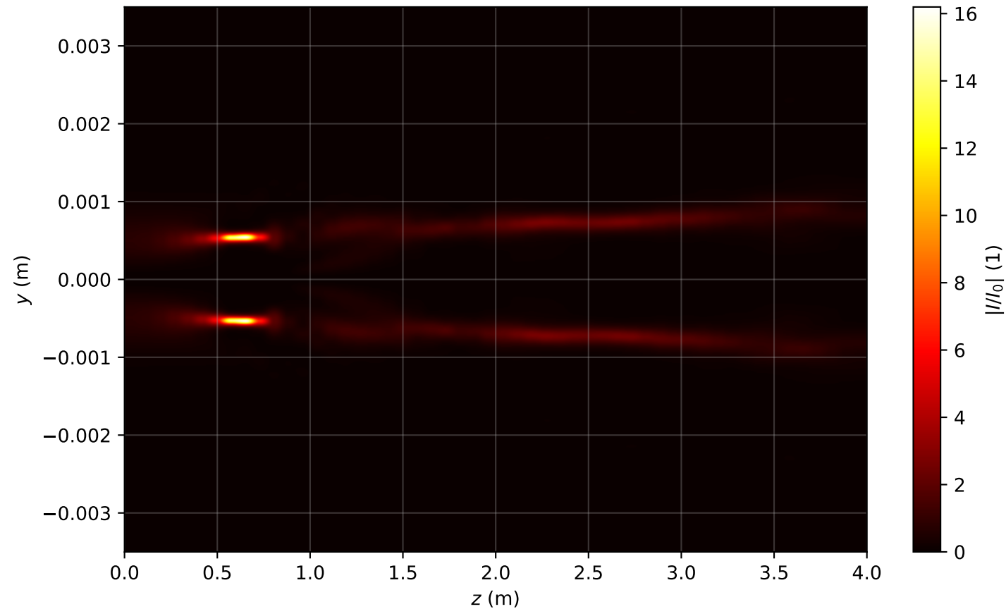
Intensity profile I(x = 0, y, z)/I_0 , P_{in}=12.0P_{cr} , artificial time
