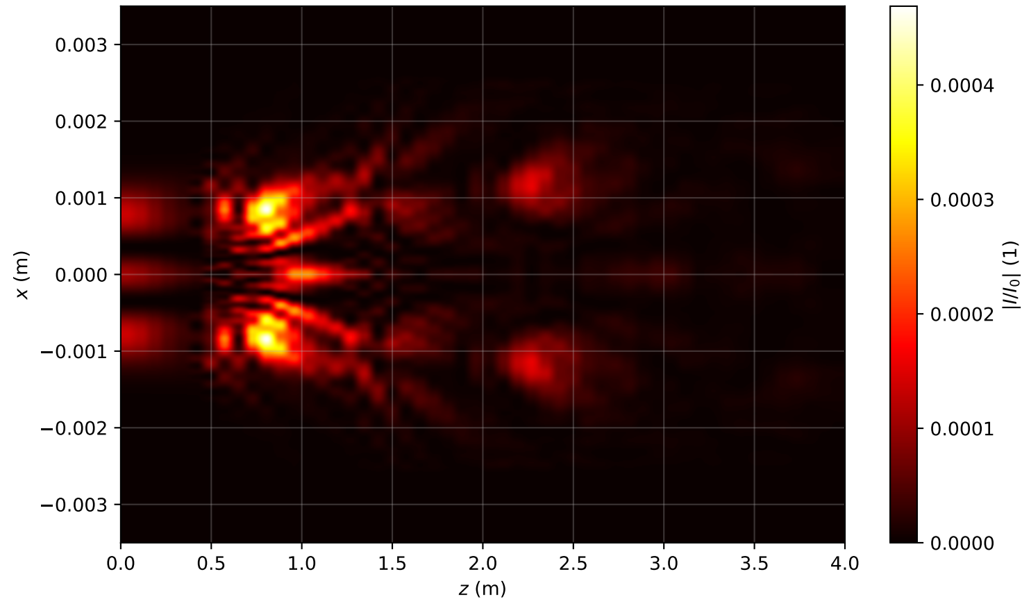
Intensity profile I(x, y = 0, z)/I_0 , P_{in}=13.0P_{cr} , artificial time
