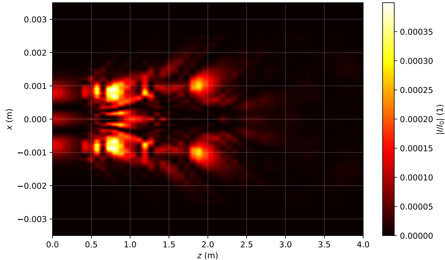
Intensity profile I(x, y = 0, z)/I_0 , P_{in}=14.0P_{cr} , artificial time
