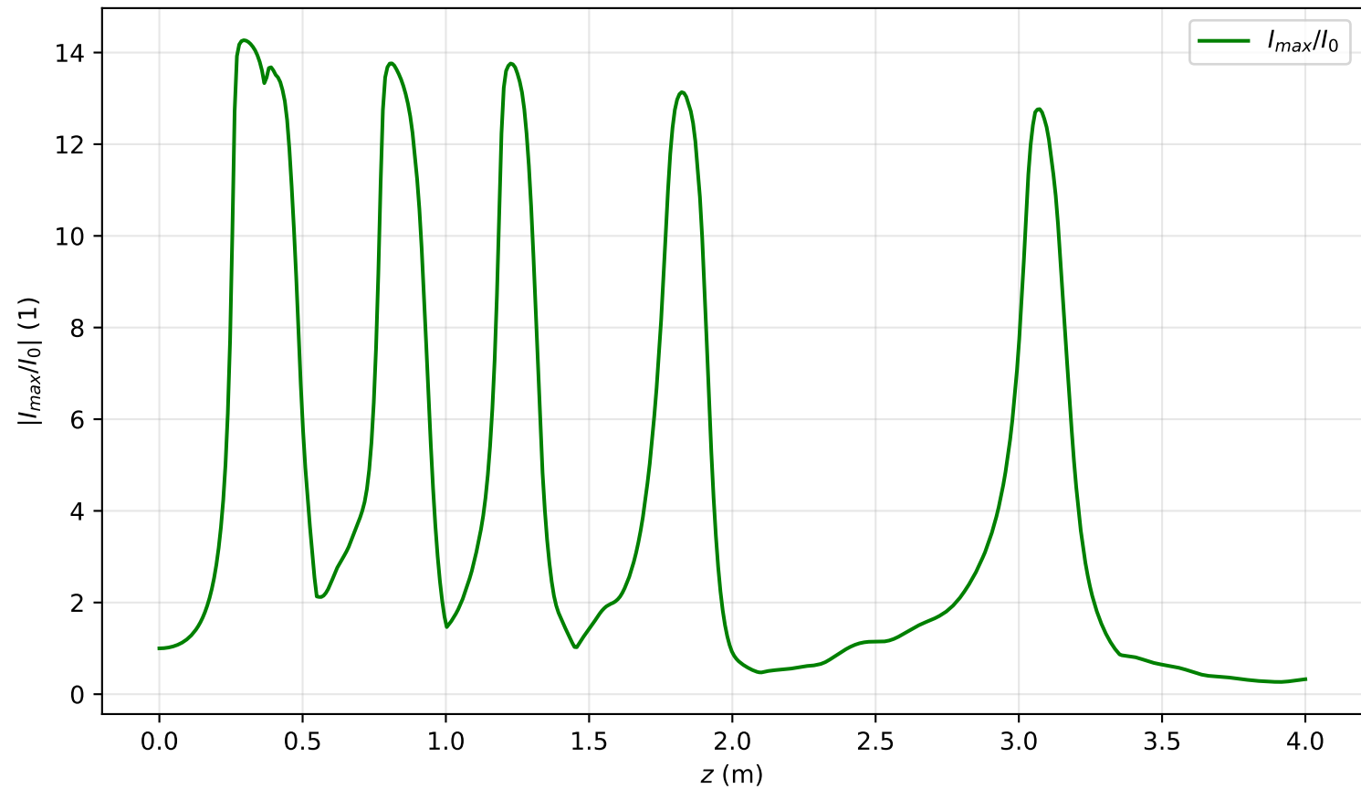
I_{\max}(x = 0, y = 0, z)/I_0 , Pin=16.0Pcr, artificial time
