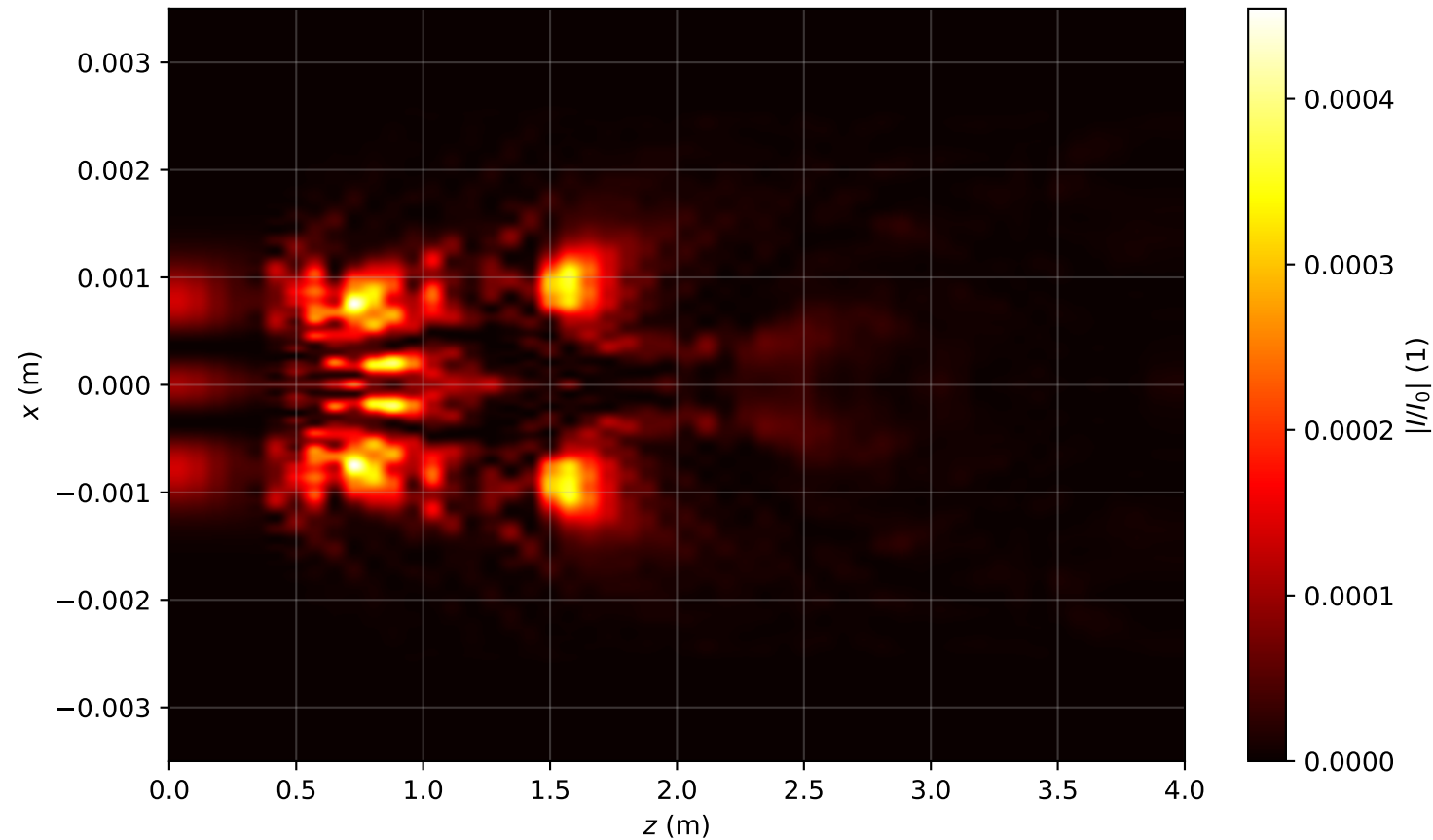
Intensity profile I(x, y = 0, z)/I_0 , P_{in}=16.0P_{cr} , artificial time
