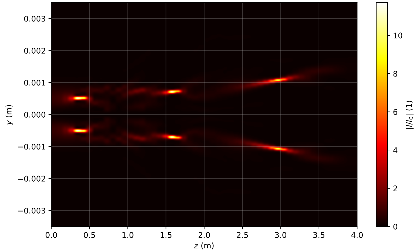
Intensity profile I(x = 0, y, z)/I_0 , P_{in}=19.0P_{cr} , artificial time
