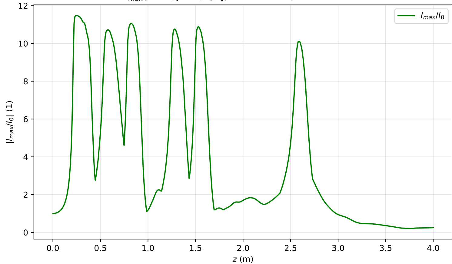
I_{\max}(x = 0, y = 0, z)/I_0 , Pin=20.0Pcr, artificial time
