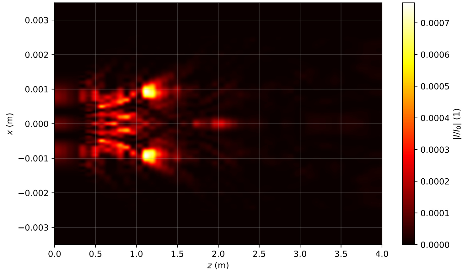
Intensity profile I(x, y = 0, z)/I_0 , P_{in}=20.0P_{cr} , artificial time
