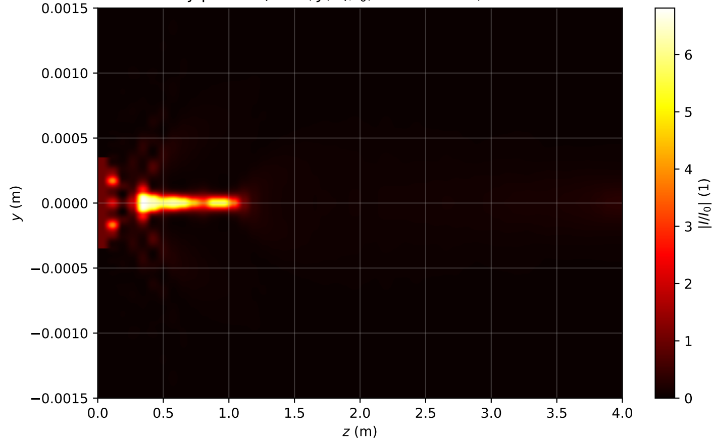
Intensity profile I(x = 0, y, z)/I_0 , P_{in}=11.0\text{Pcr} , artificial time
