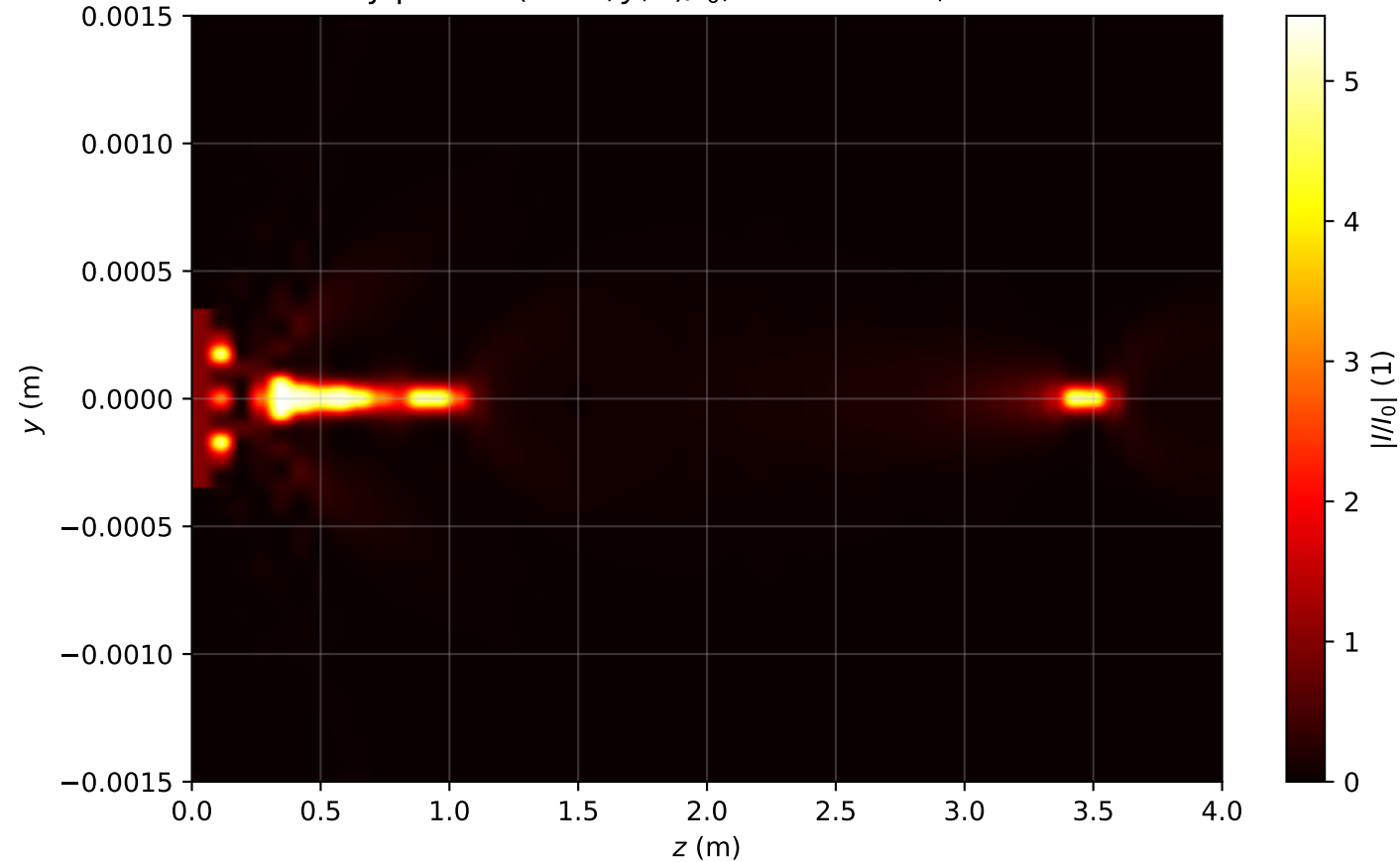
Intensity profile I(x = 0, y, z)/I_0 , P_{in}=13.0P_{cr} , artificial time
