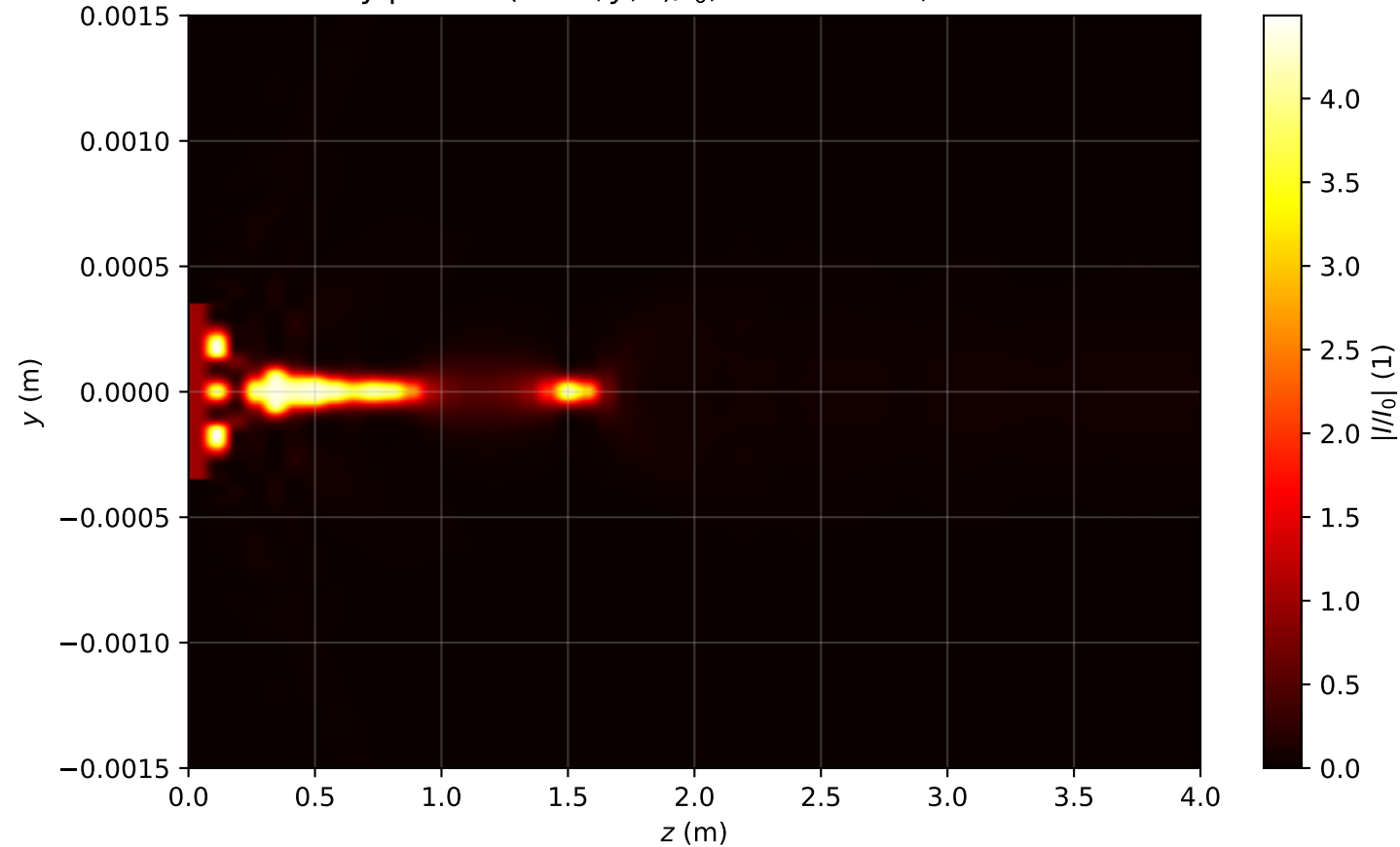
Intensity profile I(x=0, y, z)/I_0 , P_{in}=16.0P_{cr} , artificial time
