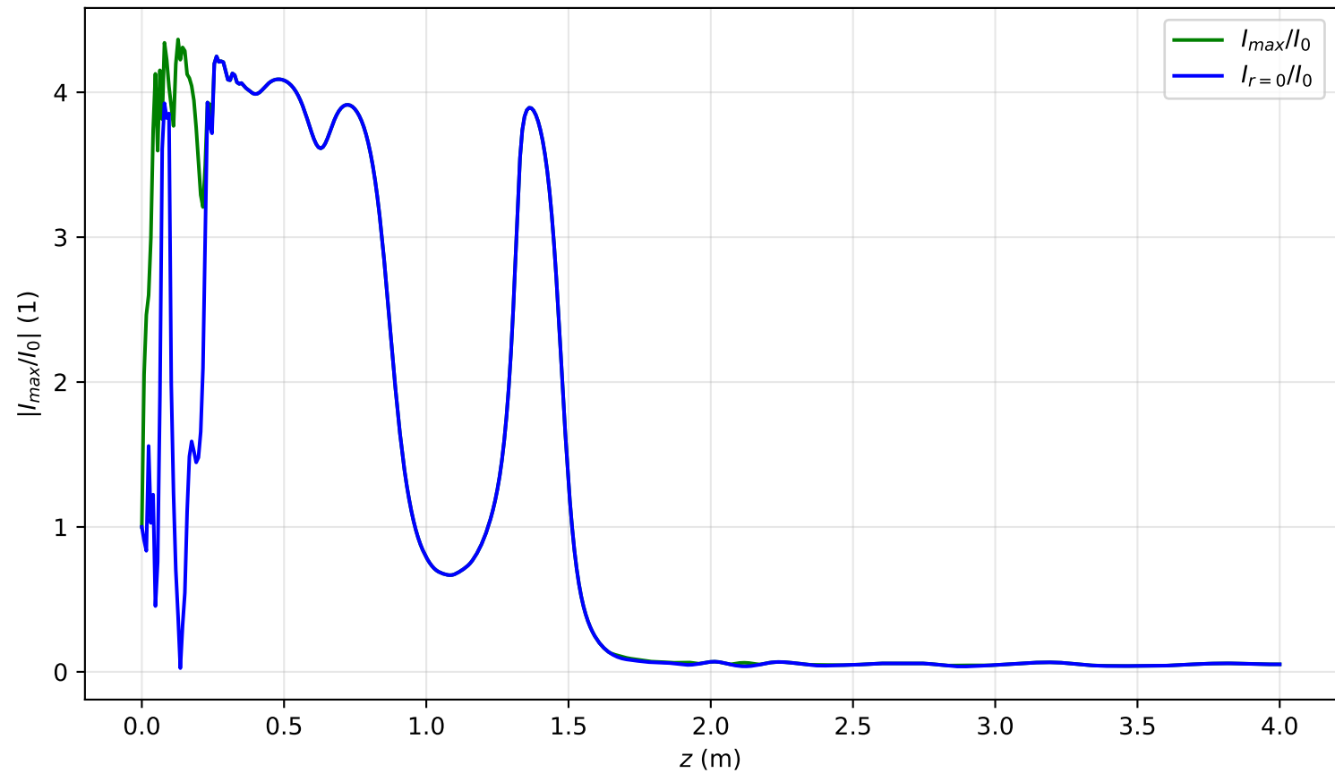
I_{\max}(x = 0, y = 0, z)/I_0 , Pin=17.0Pcr, artificial time
