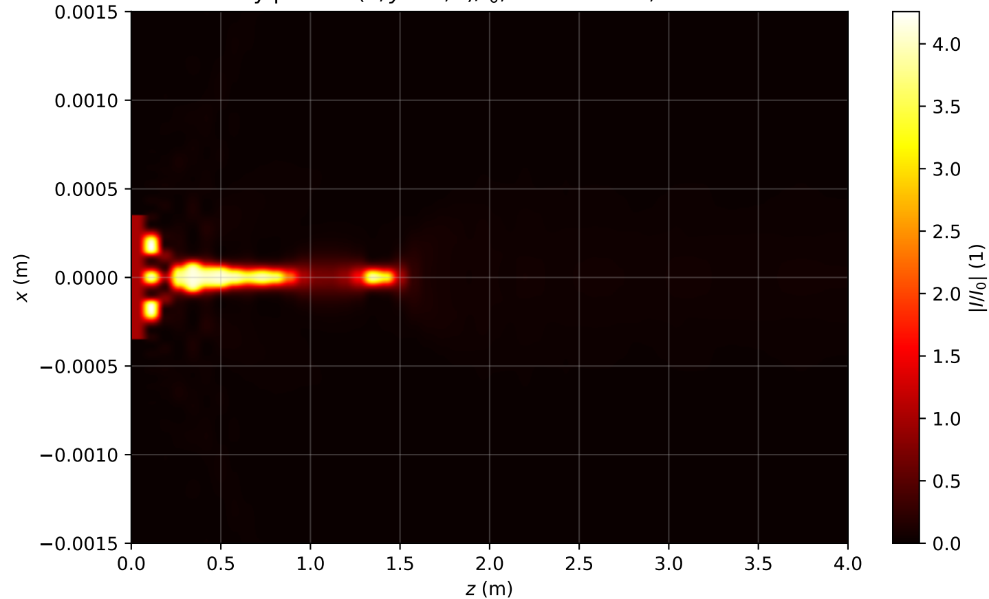
Intensity profile I(x, y = 0, z)/I_0 , P_{in}=17.0\text{Pcr} , artificial time
