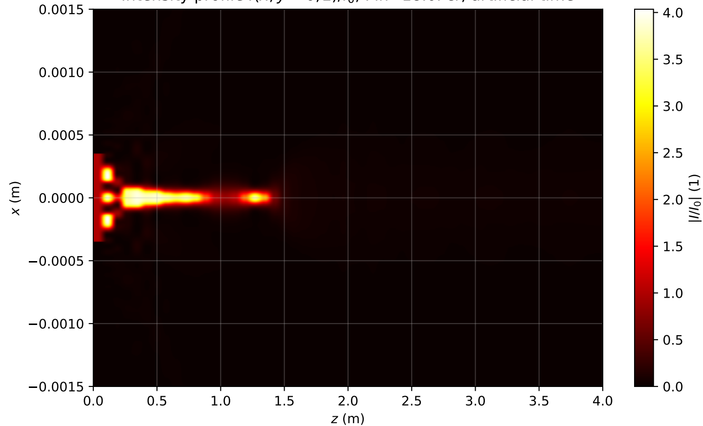
Intensity profile I(x, y = 0, z)/I_0 , P_{in}=18.0P_{cr} , artificial time
