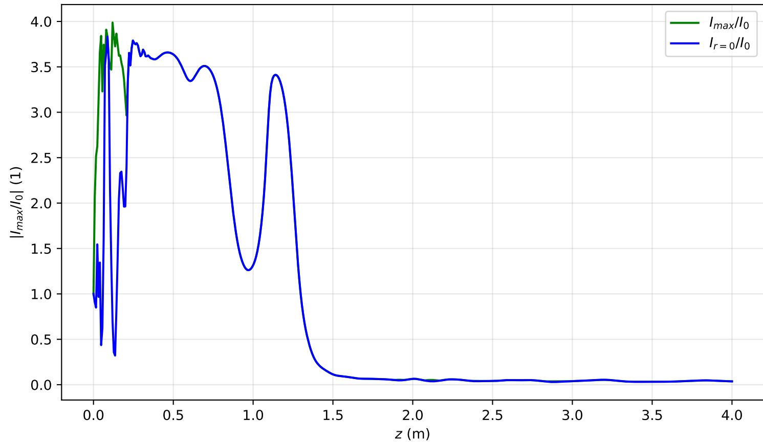
I_{\max}(x=0, y=0, z)/I_0 , Pin=19.0Pcr, artificial time
