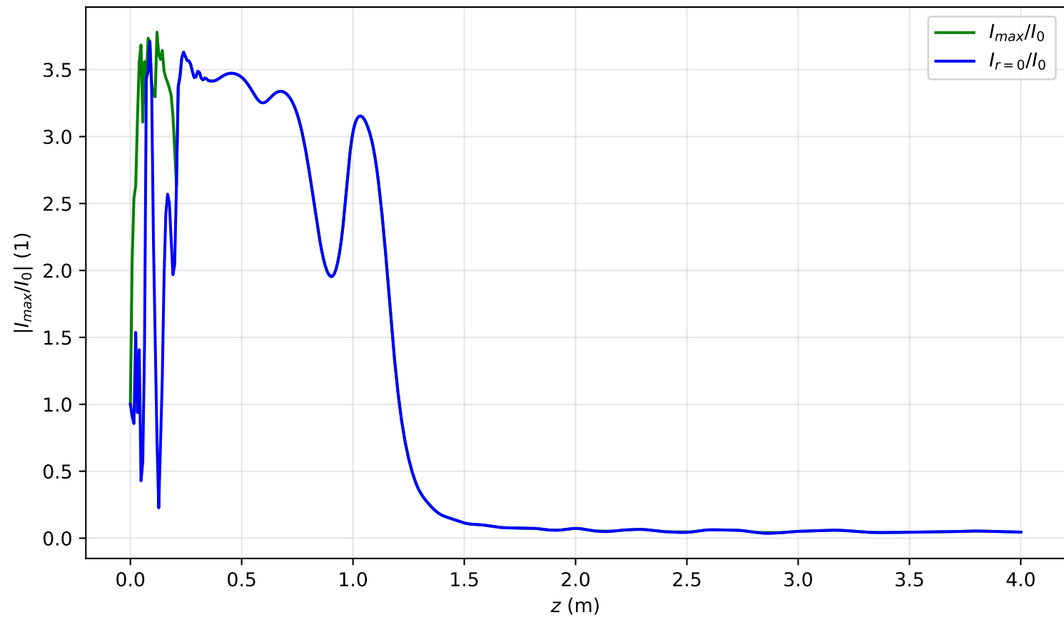
I_{max}(x = 0, y = 0, z)/I_0 , Pin=20.0Pcr, artificial time
