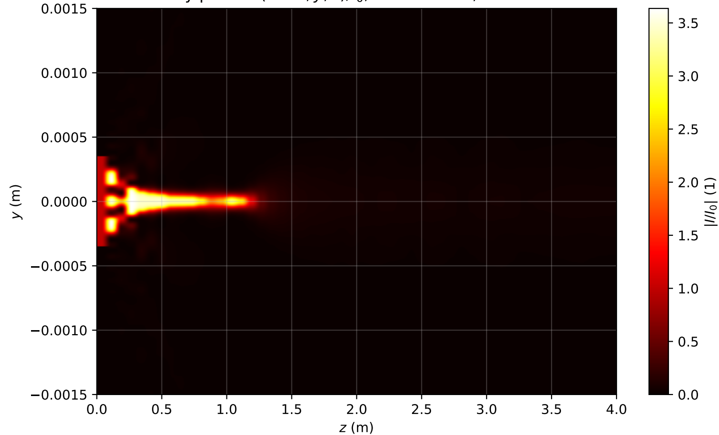
Intensity profile I(x=0, y, z)/I_0 , P_{in}=20.0P_{cr} , artificial time
