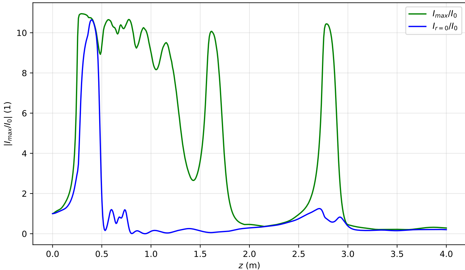
I_{\max}(x = 0, y = 0, z)/I_0 , \text{Pin}=10.1\text{Pcr} , noisy input, artificial time
