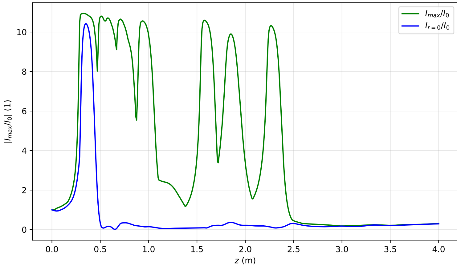
I_{\max}(x = 0, y = 0, z)/I_0 , \text{Pin}=10.2\text{Pcr} , noisy input, artificial time
