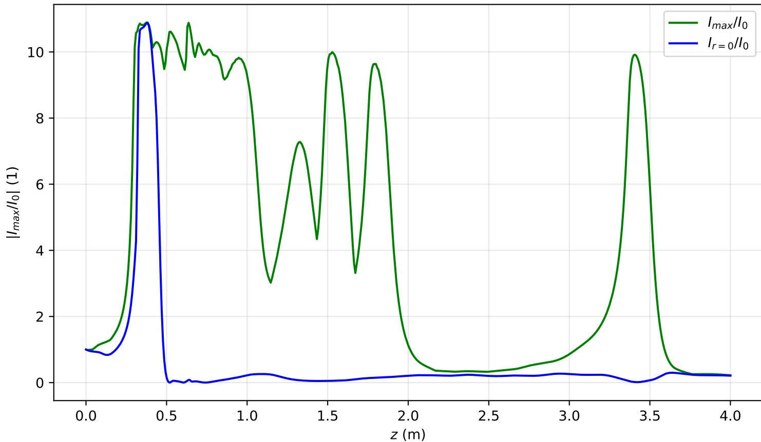
I_{max}(x = 0, y = 0, z)/I_0 , P_{in}=10.3P_{cr} , noisy input, artificial time
