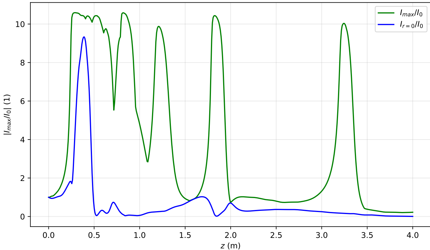
I_{max}(x = 0, y = 0, z)/I_0 , P_{in}=10.4P_{cr} , noisy input, artificial time
