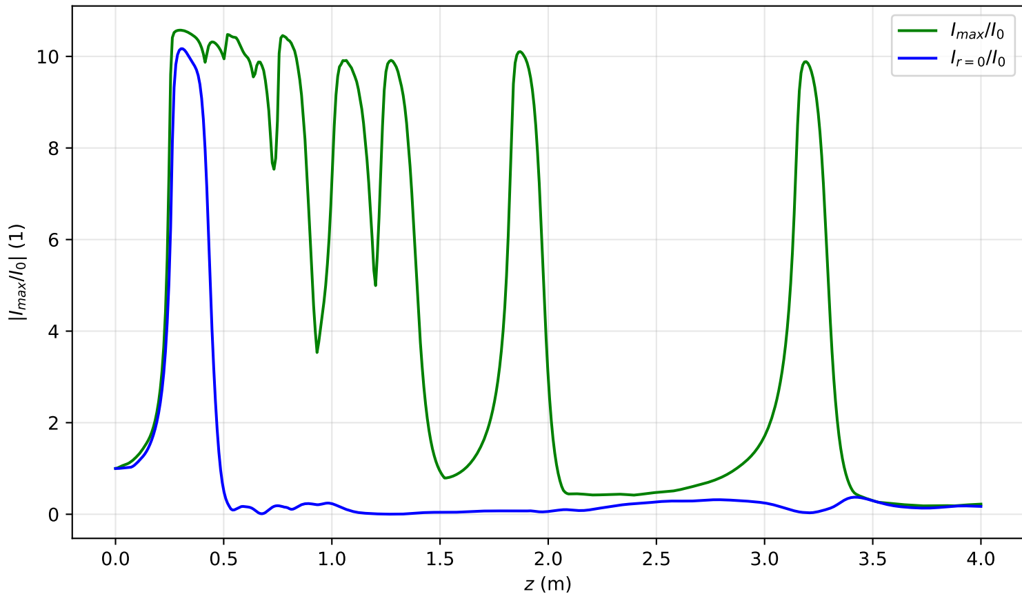
I_{max}(x = 0, y = 0, z)/I_0 , P_{in}=10.5P_{cr} , noisy input, artificial time
