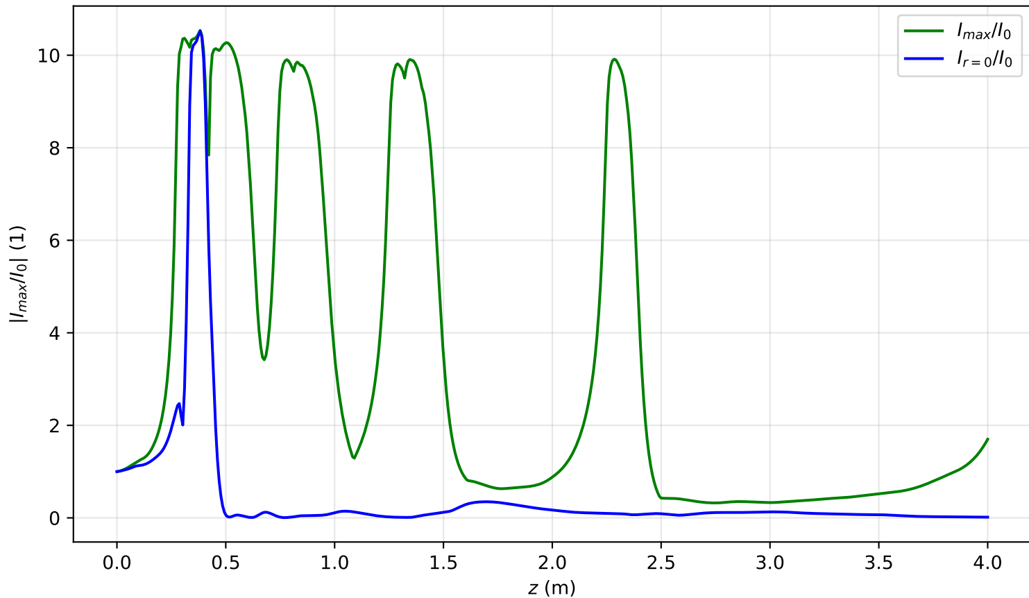
I_{max}(x = 0, y = 0, z)/I_0 , Pin=10.7Pcr, noisy input, artificial time
