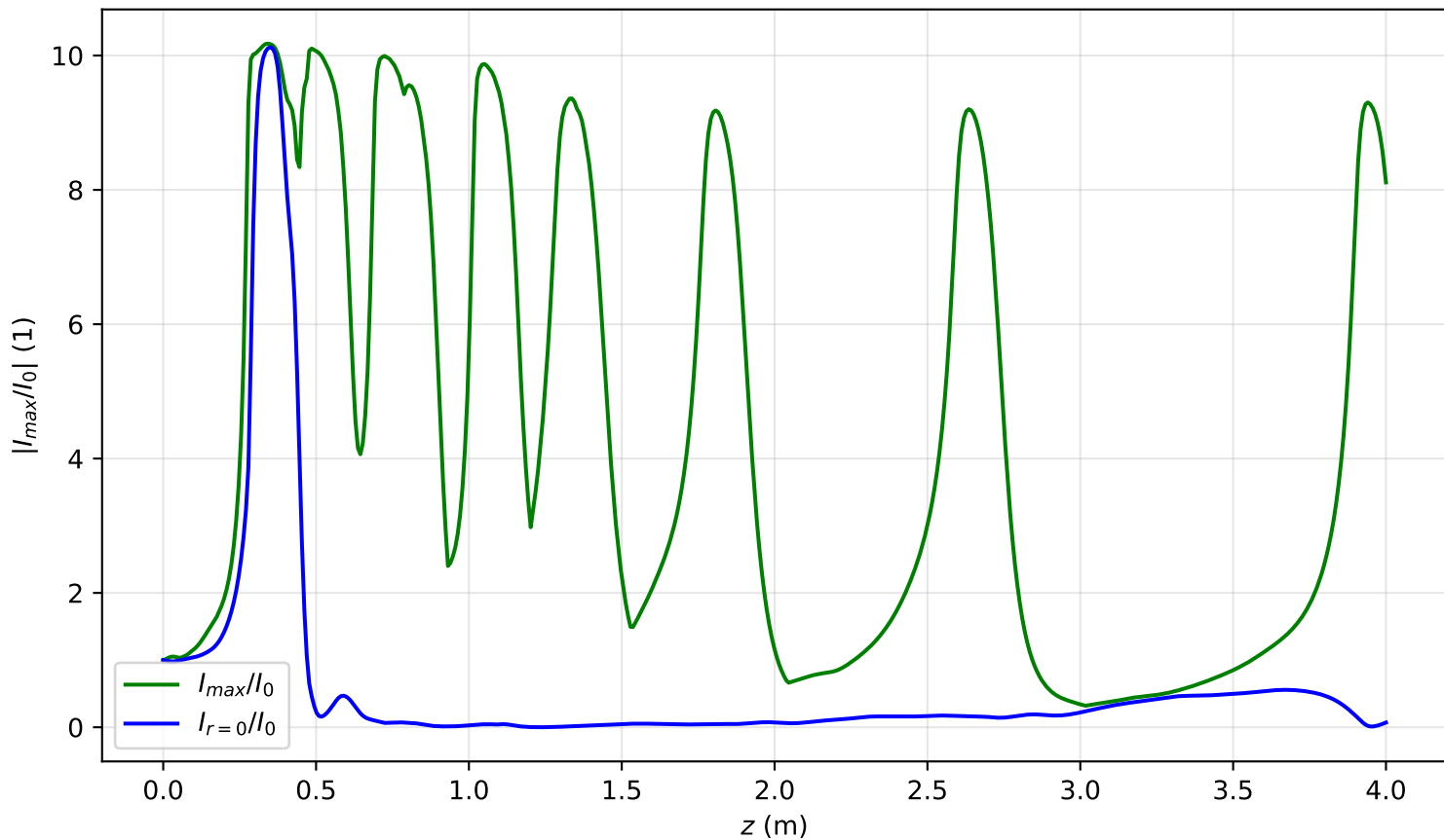
I_{\max}(x = 0, y = 0, z)/I_0 , \text{Pin}=10.9\text{Pcr} , noisy input, artificial time
