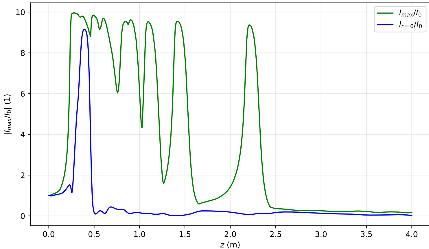
I_{\max}(x = 0, y = 0, z)/I_0 , Pin=11.1Pcr, noisy input, artificial time
