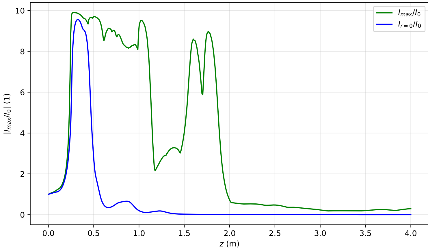
I_{max}(x = 0, y = 0, z)/I_0 , Pin=11.2Pcr, noisy input, artificial time
