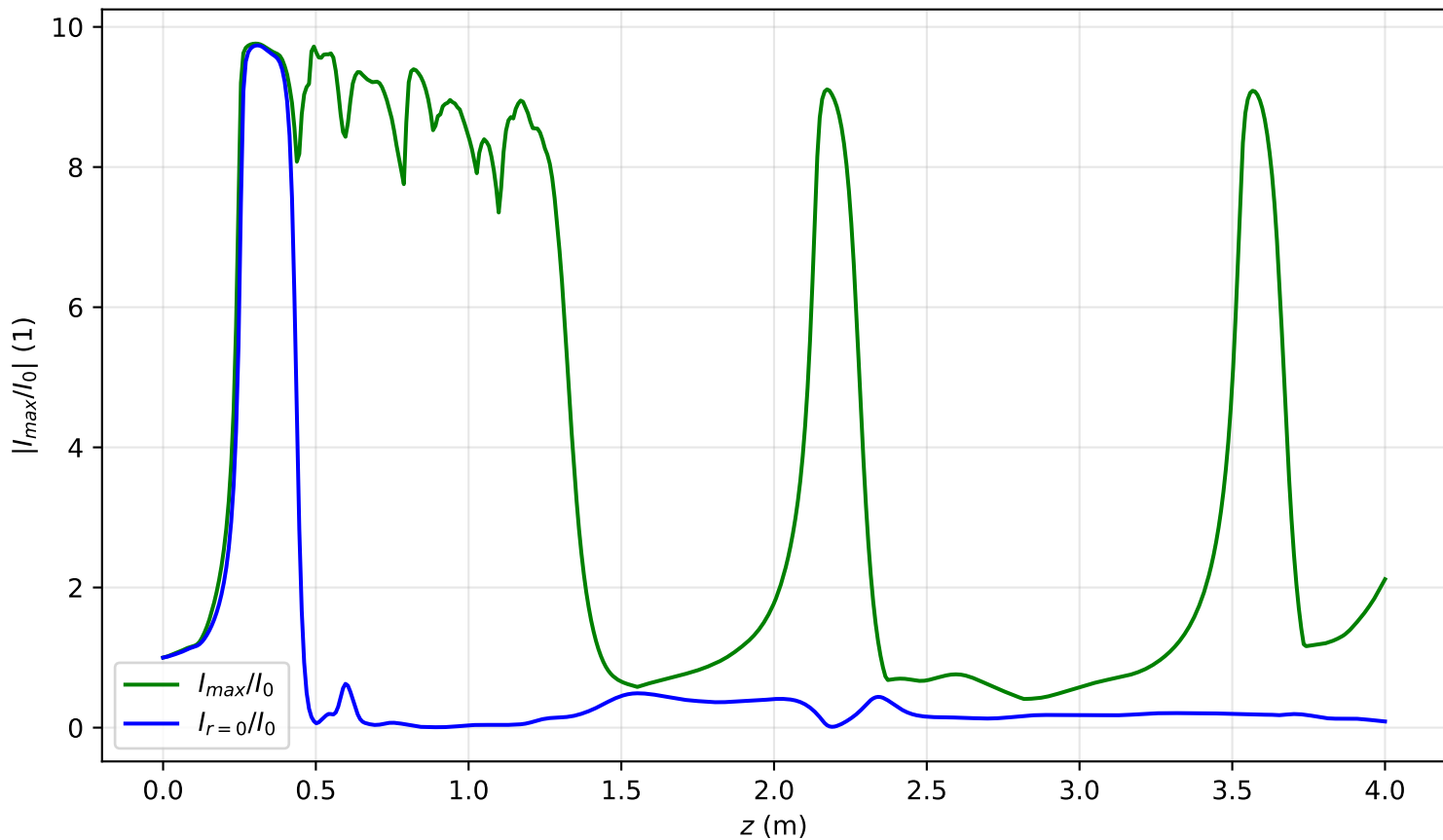
I_{\max}(x = 0, y = 0, z)/I_0 , P_{\text{in}}=11.4\text{Pcr} , noisy input, artificial time
