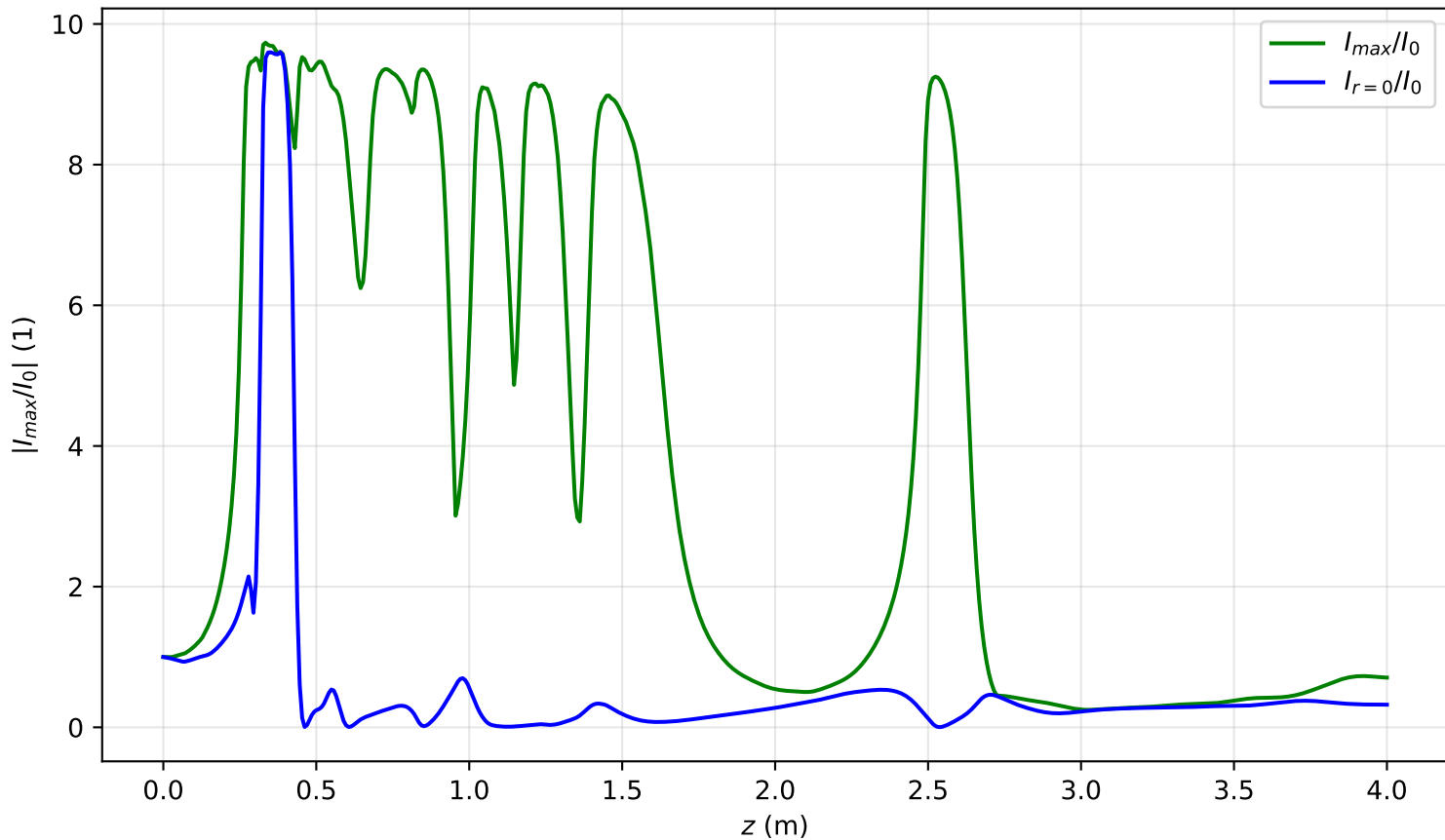
I_{\max}(x=0, y=0, z)/I_0 , P_{\text{in}}=11.5\text{Pcr} , noisy input, artificial time
