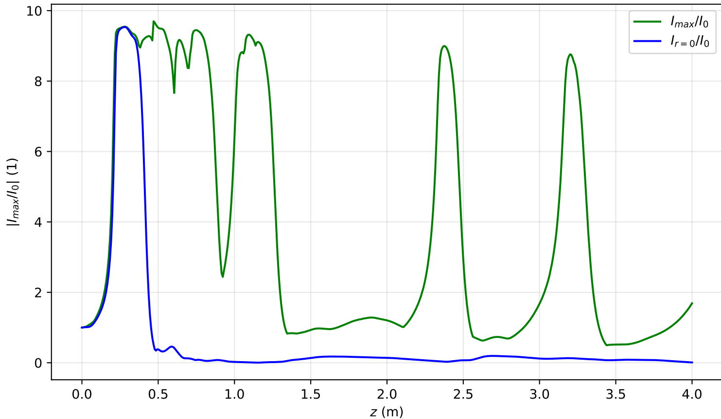
I_{max}(x = 0, y = 0, z)/I_0 , P_{in}=11.6P_{cr} , noisy input, artificial time
