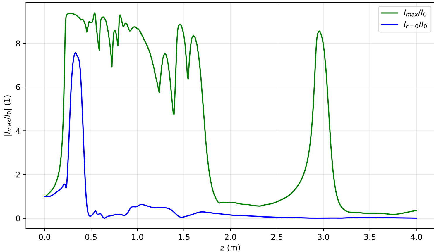
I_{max}(x = 0, y = 0, z)/I_0 , Pin=11.8Pcr, noisy input, artificial time
