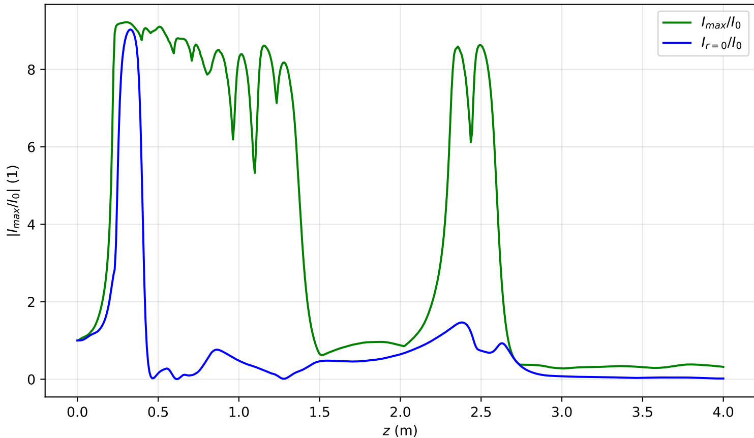
I_{max}(x = 0, y = 0, z)/I_0 , Pin=12.0Pcr, noisy input, artificial time
