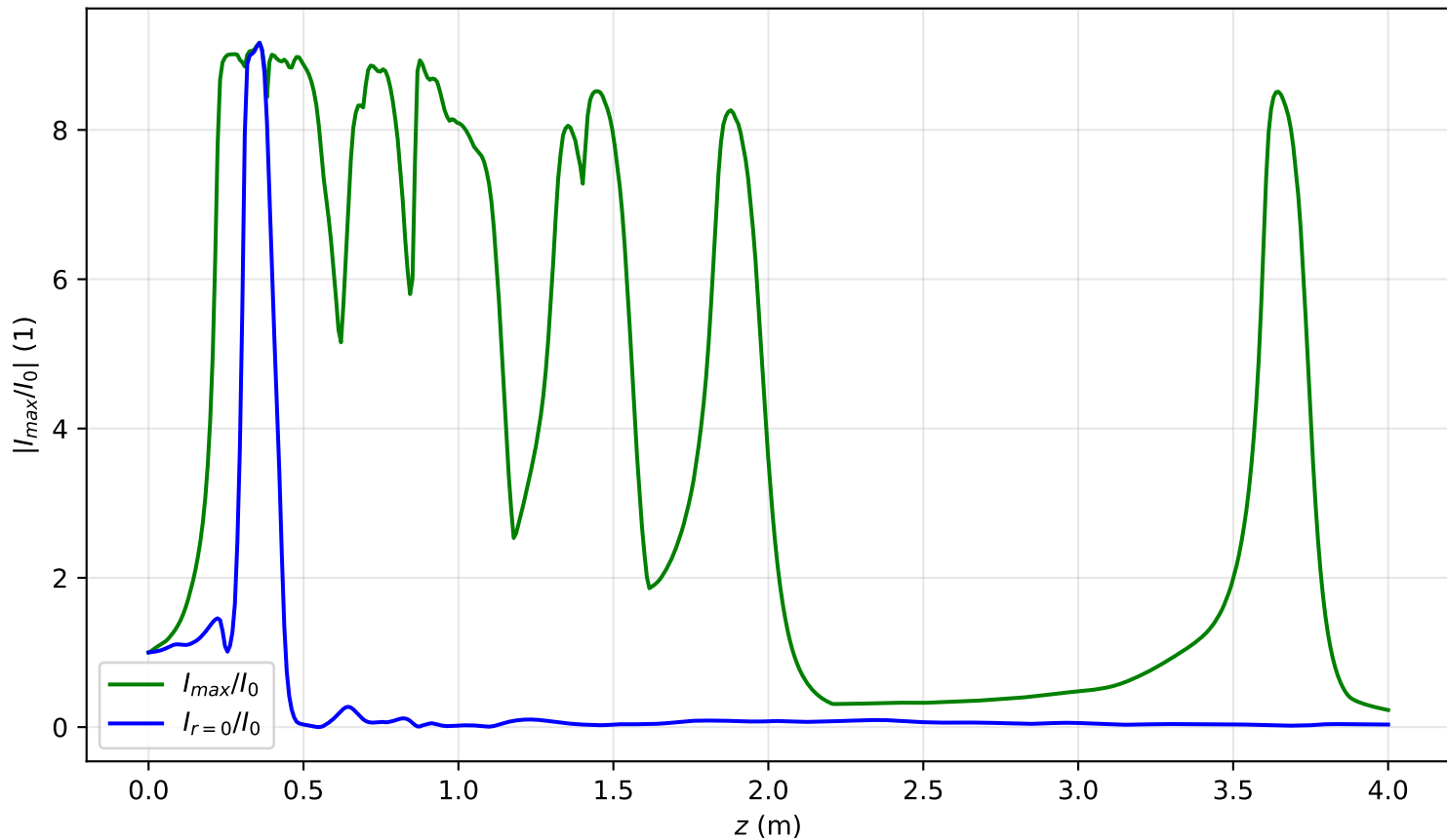
I_{\max}(x = 0, y = 0, z)/I_0 , P_{\text{in}}=12.2\text{Pcr} , noisy input, artificial time
