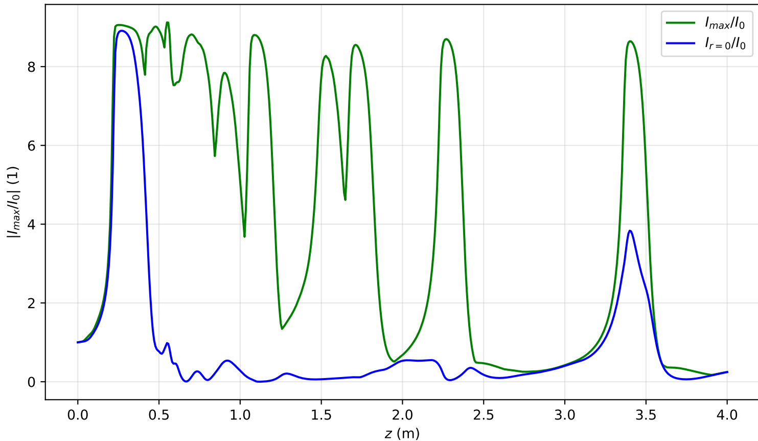
I_{max}(x = 0, y = 0, z)/I_0 , Pin=12.3Pcr, noisy input, artificial time
