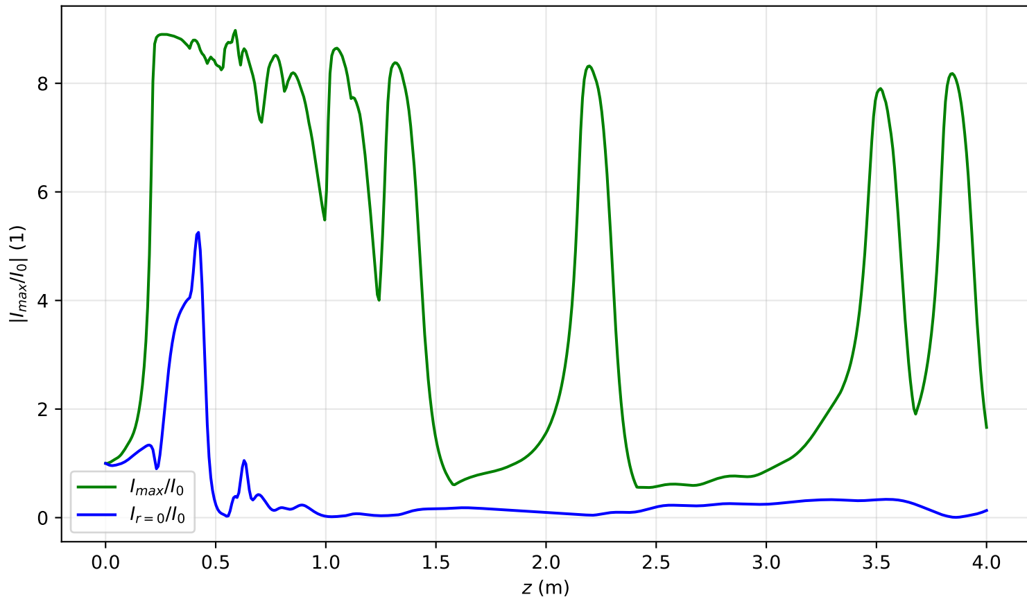
I_{\max}(x = 0, y = 0, z)/I_0 , P_{\text{in}}=12.4\text{Pcr} , noisy input, artificial time
