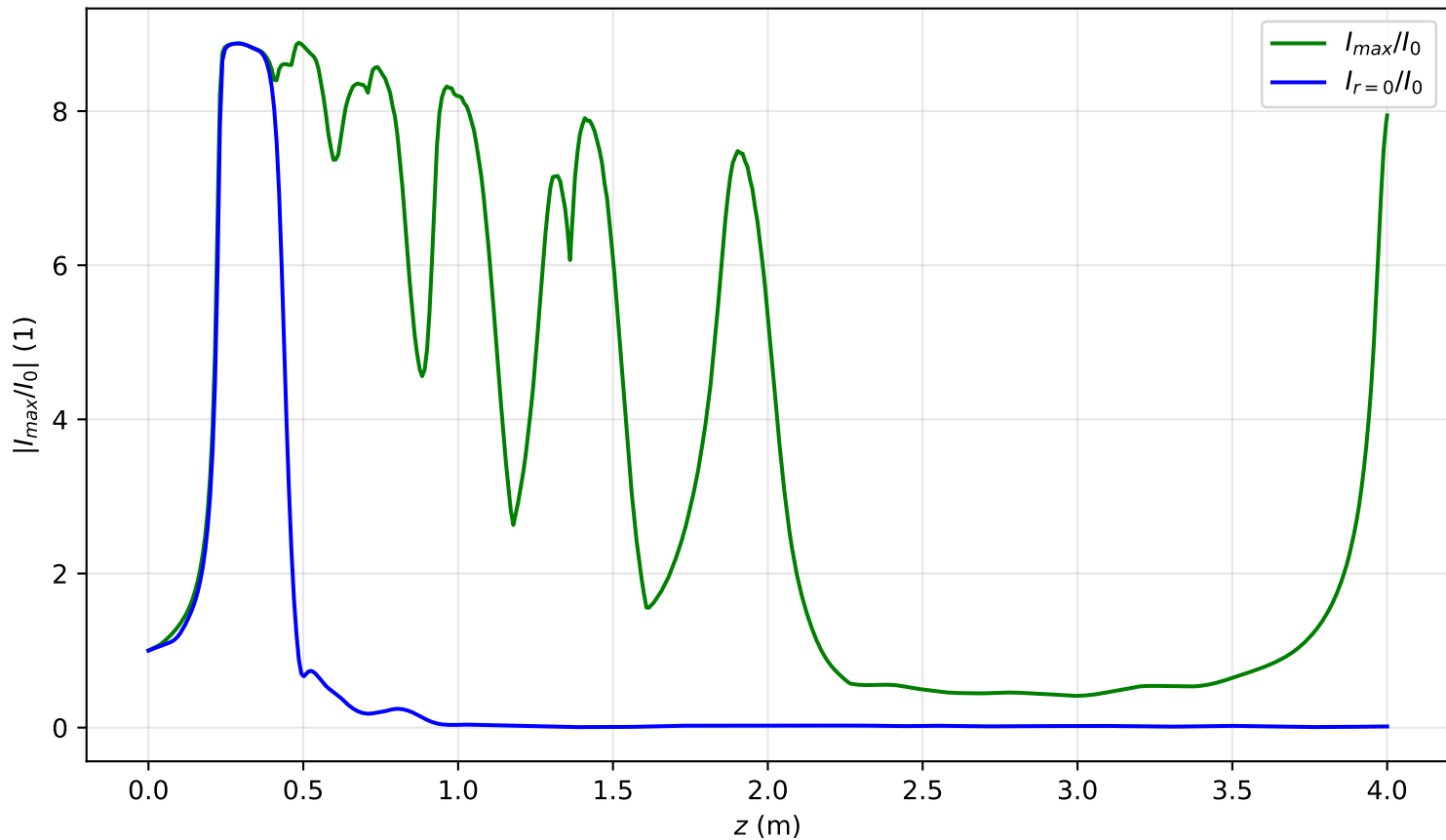
I_{\max}(x = 0, y = 0, z)/I_0 , Pin=12.5Pcr, noisy input, artificial time
