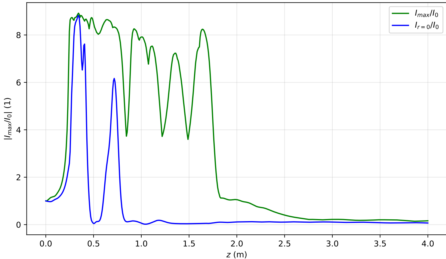
I_{max}(x = 0, y = 0, z)/I_0 , Pin=12.6Pcr, noisy input, artificial time
