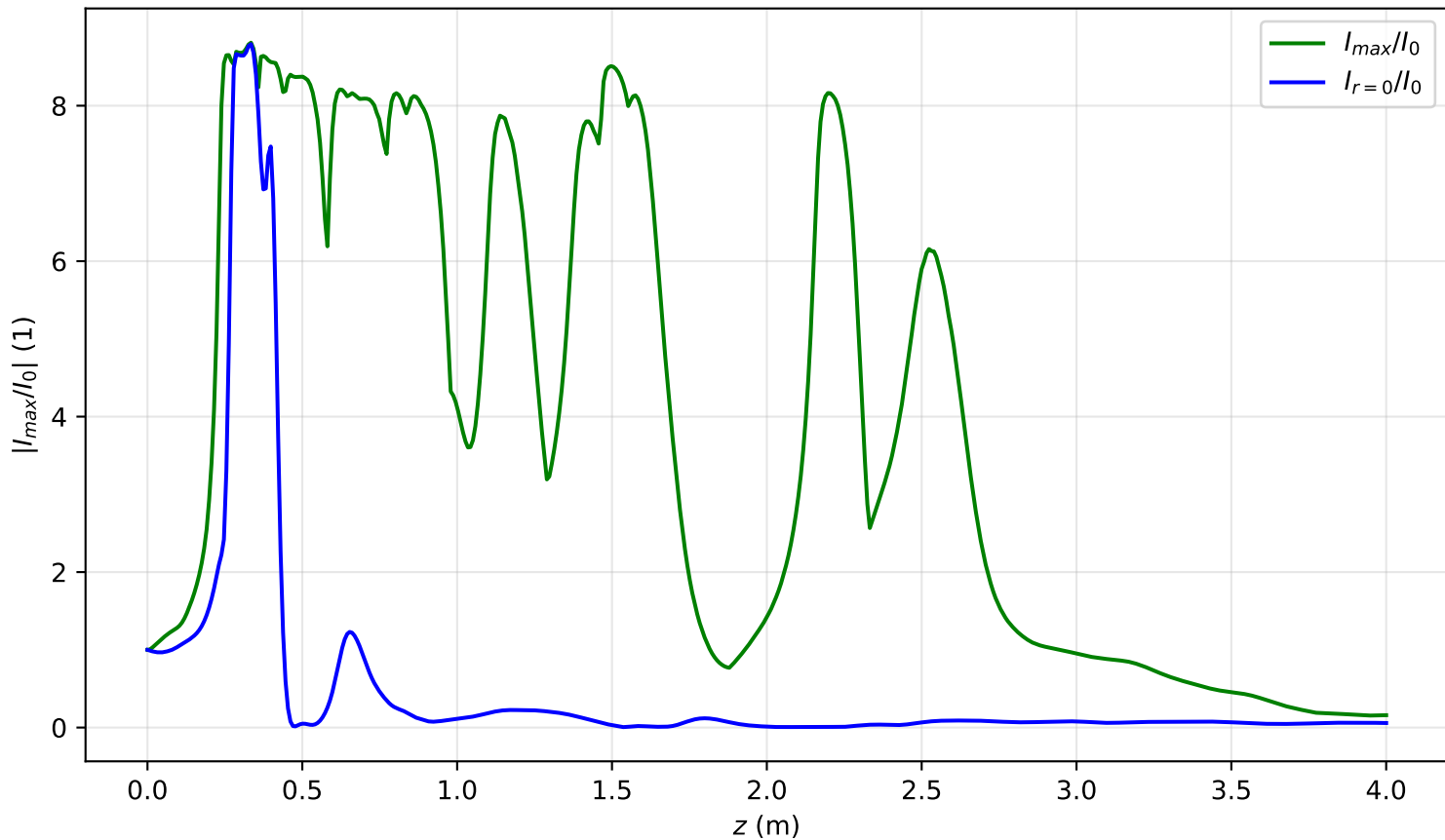
I_{max}(x = 0, y = 0, z)/I_0 , P_{in}=12.7P_{cr} , noisy input, artificial time
