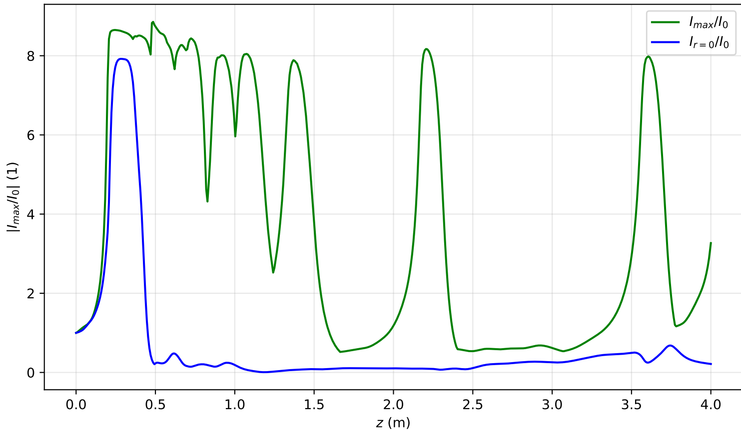
I_{max}(x = 0, y = 0, z)/I_0 , P_{in}=12.8P_{cr} , noisy input, artificial time
